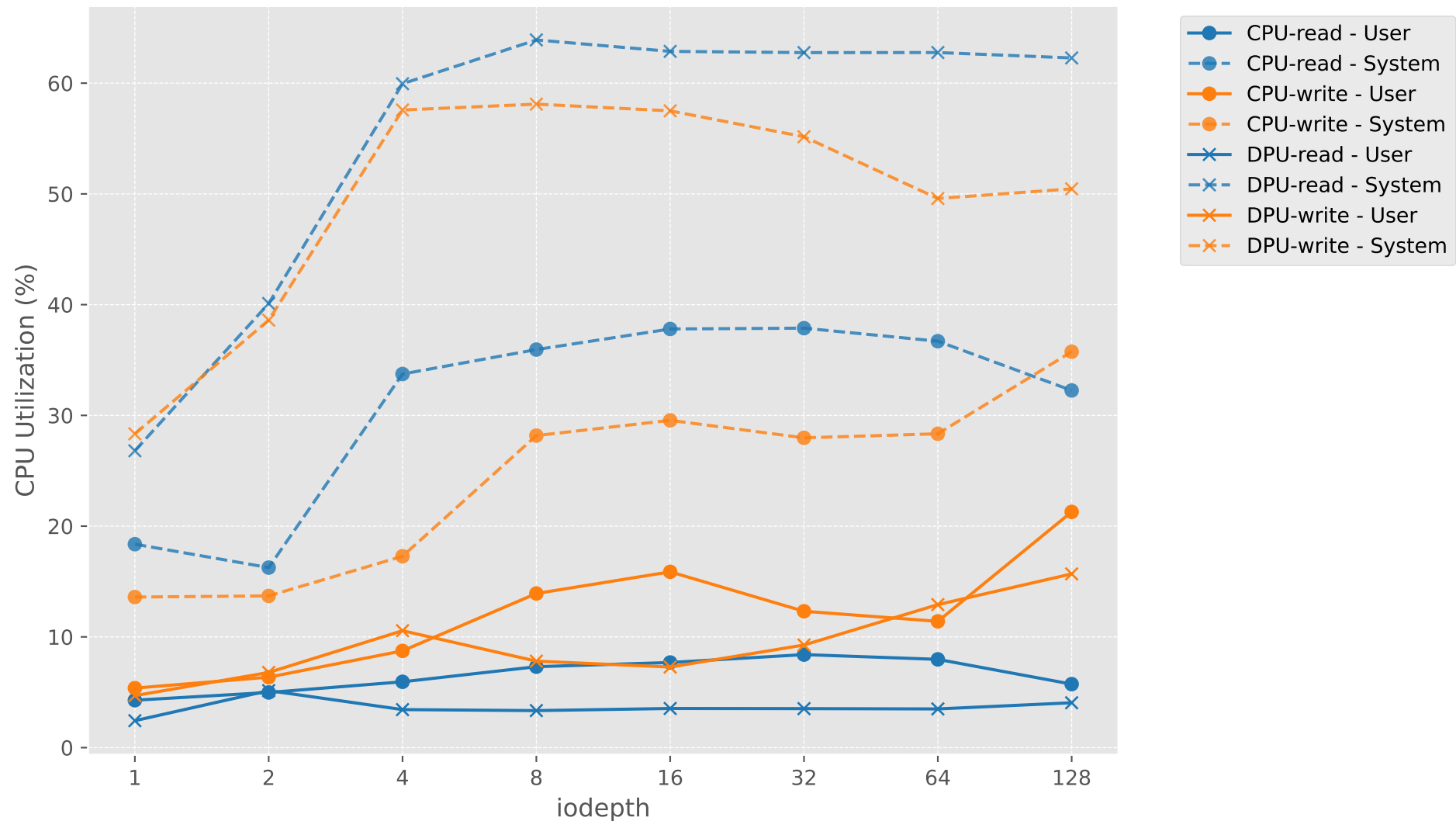
CPU Utilization vs iodepth (Sequential)
